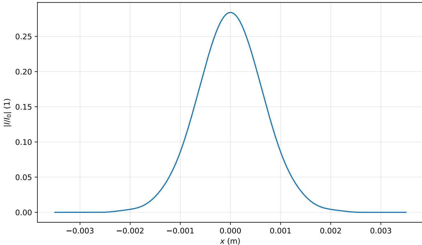
Intensity profile I(x, y = 0, z = 3.981m)/I_0 , P_{in}=0.3P_{cr} , artificial time
